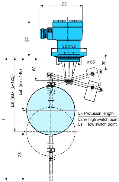
Top mounted with adjustable switch differential ■ MKA-230
