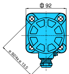
Connection flange □
