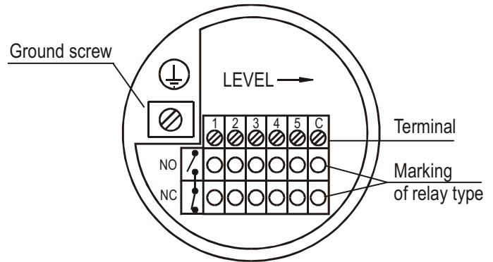
Figure 3.: Housing with removed cover
