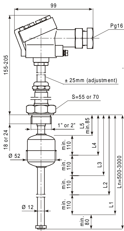
Figure 2.: Dimensions of the Ex version
